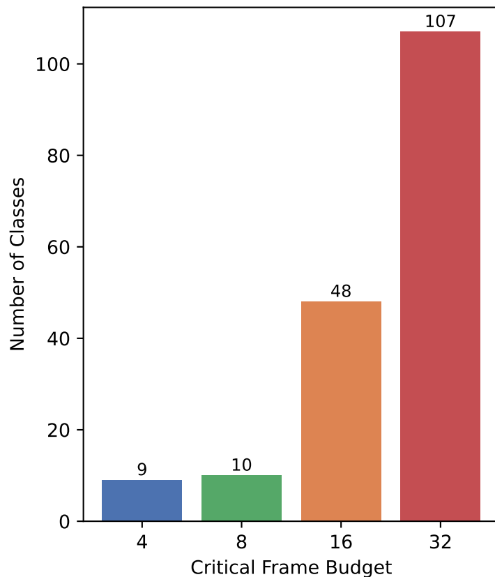
Critical Budget Distribution ViViT on SSV2
