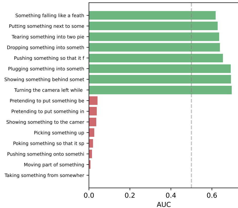
Lowest (red) & Highest (green) AUC Classes ViViT on SSV2
