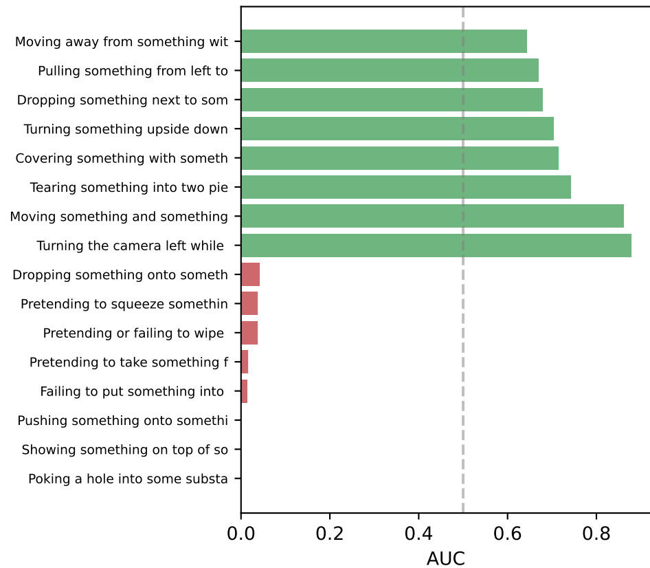
Lowest (red) & Highest (green) AUC Classes R3D-18 on SSV2
