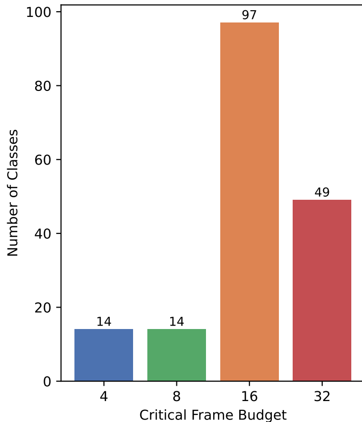
Critical Budget Distribution R3D-18 on SSV2
