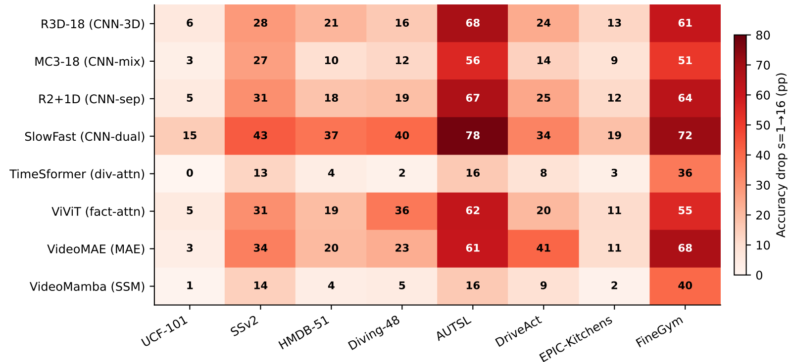
Temporal Aliasing Sensitivity — Accuracy Drop (stride 1→16, coverage=100%)
