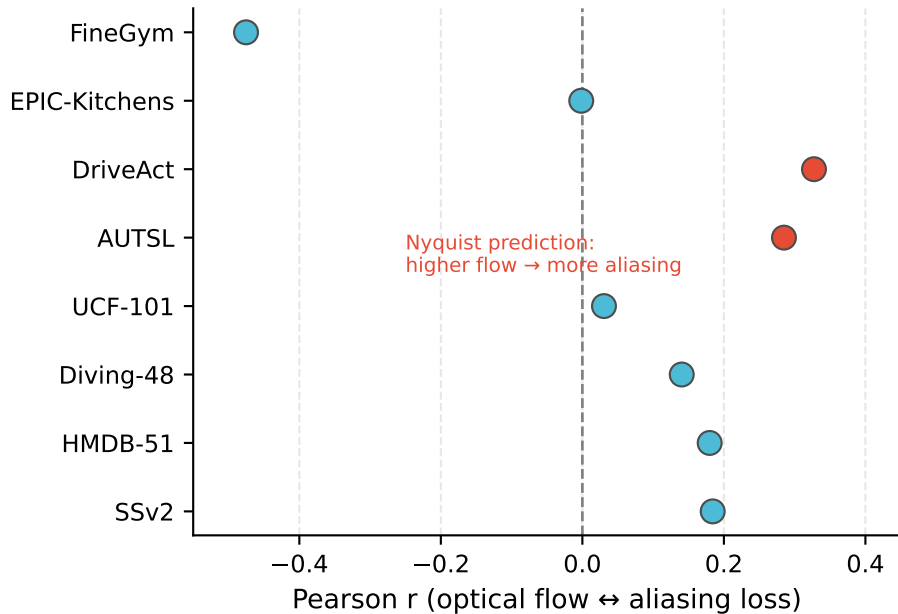
Spectral Correlation (flow magnitude vs aliasing sensitivity)
