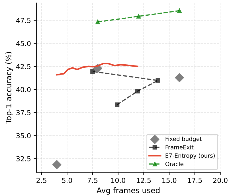
TimeSformer / SSv2
