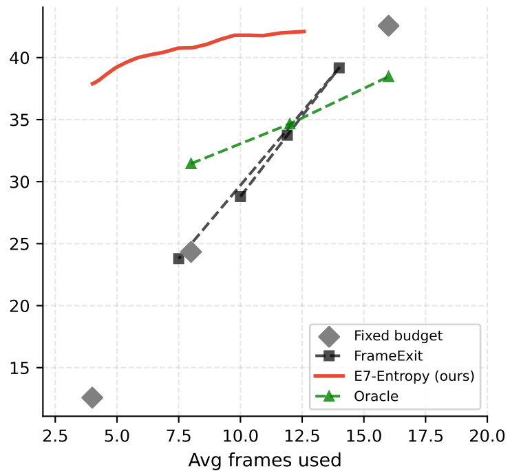
R2Plus1D / SSv2
