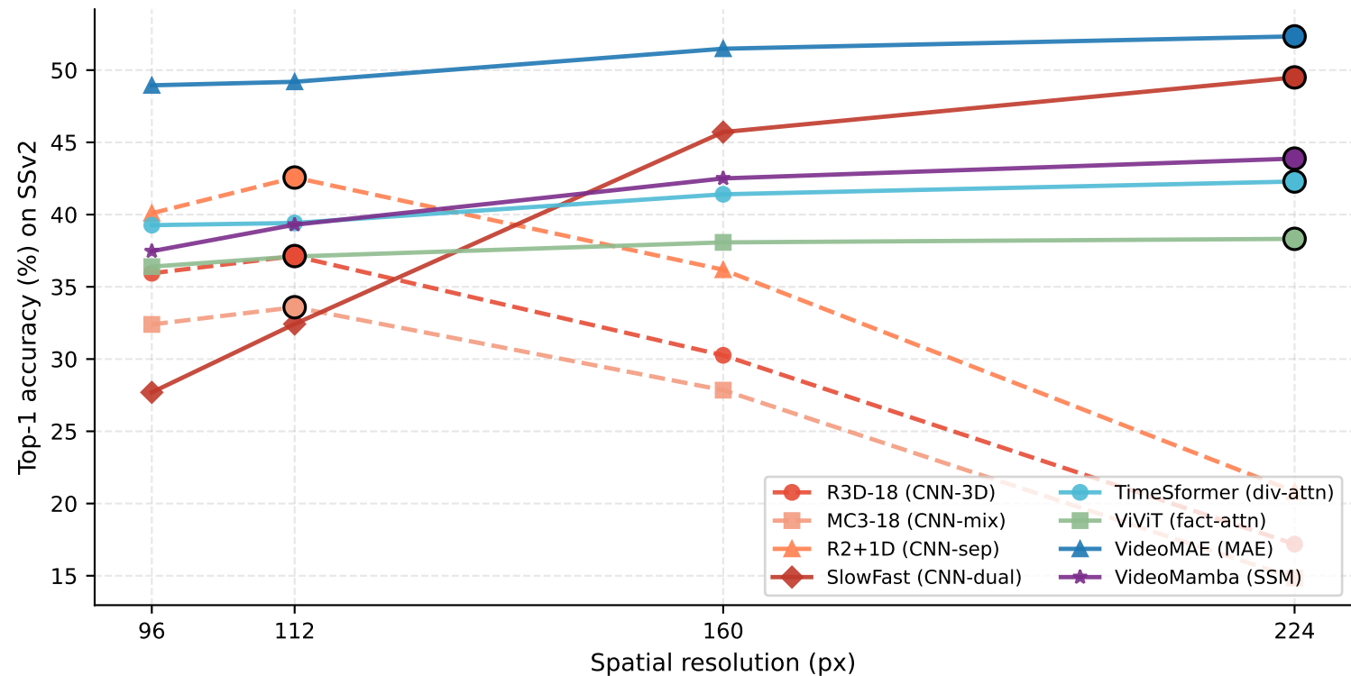
Spatial Aliasing — Accuracy vs Resolution (SSv2) Filled markers = native resolution; dashed = CNN (native 112px)
