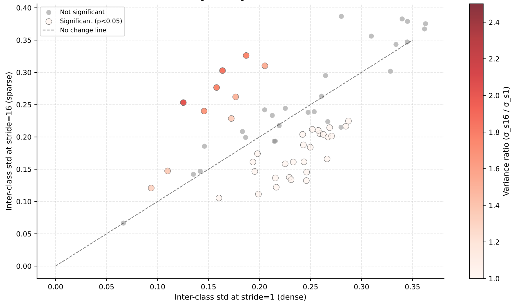
Stride increases inter-class accuracy variance (Levene test) Points above diagonal = higher variance at stride=16
