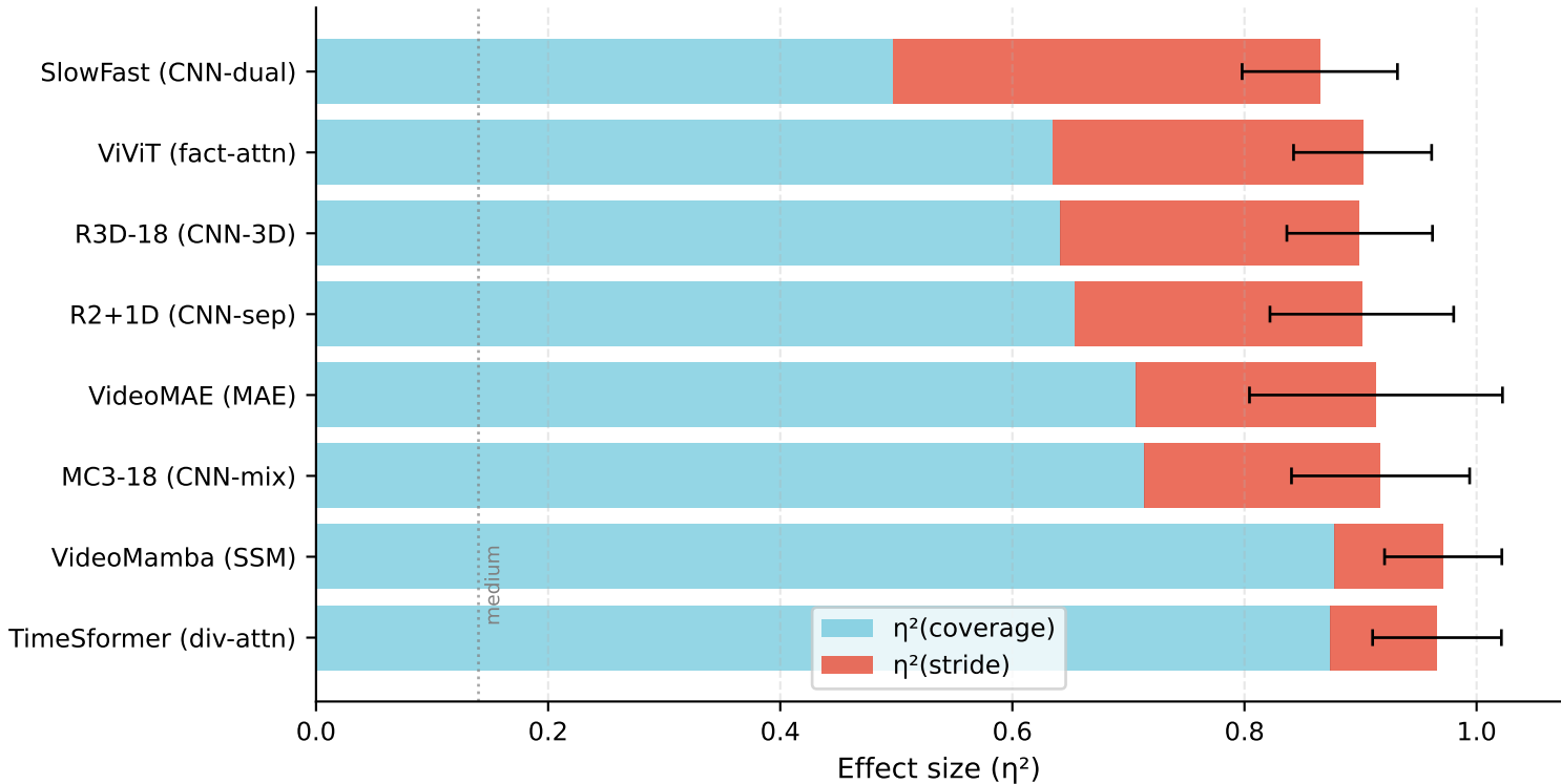
ANOVA Effect Sizes \eta^2(\text{stride}) + \eta^2(\text{coverage}) per model (avg \pm std across datasets)
