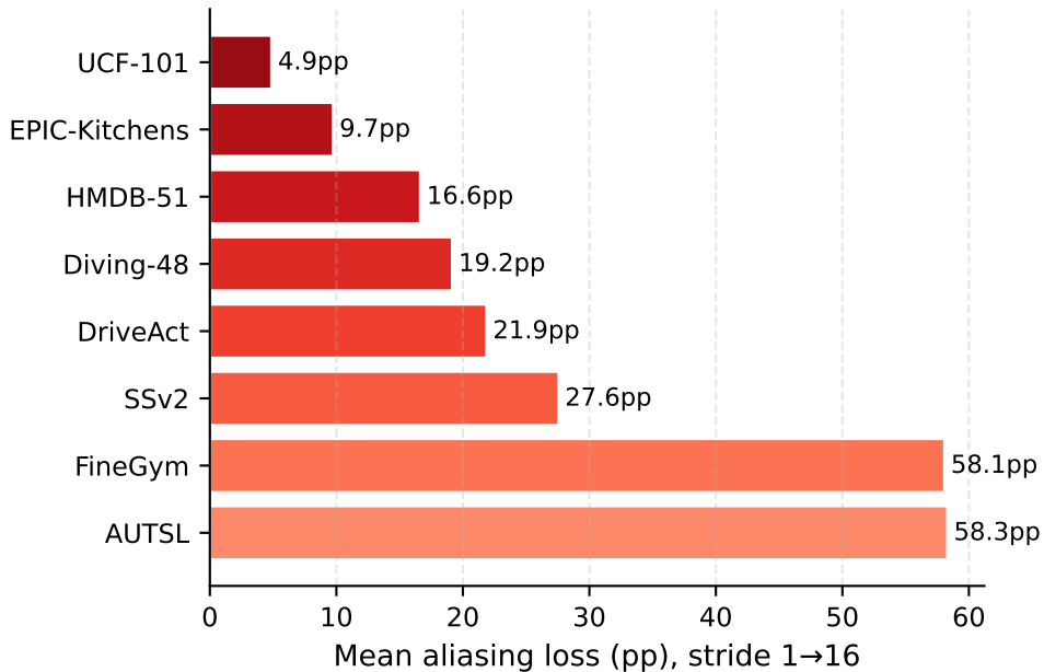
Fig 3a: TDS Ranking (avg across 8 architectures)
