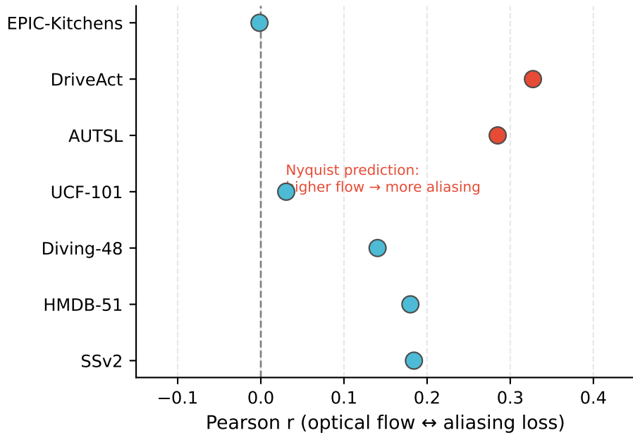
Fig 3b: Spectral Correlation (flow magnitude vs aliasing sensitivity)
