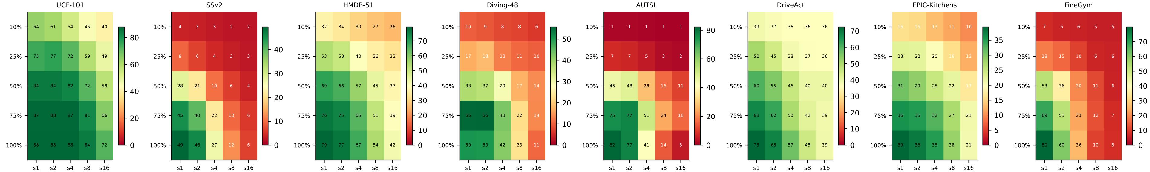
Sup1: SlowFast (CNN-dual) — Coverage×Stride accuracy (%) per dataset
