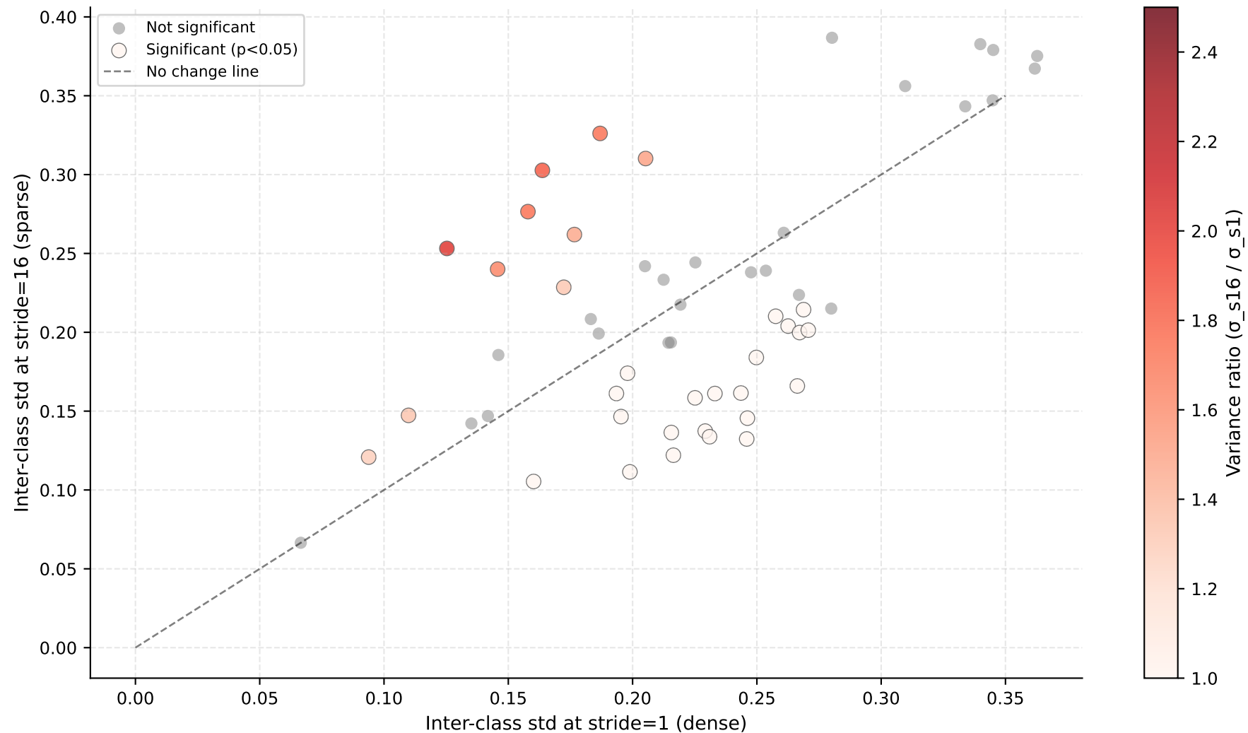
Sup2: E2 — Stride increases inter-class accuracy variance (Levene test)
