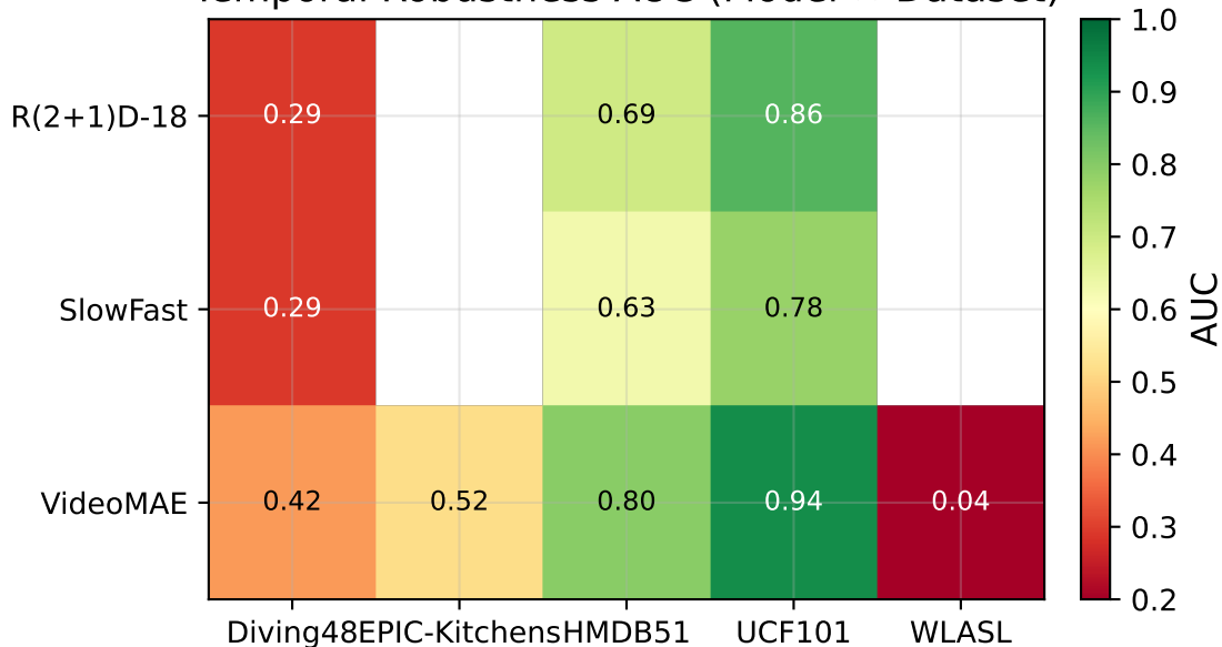
Temporal Robustness AUC (Model × Dataset)
