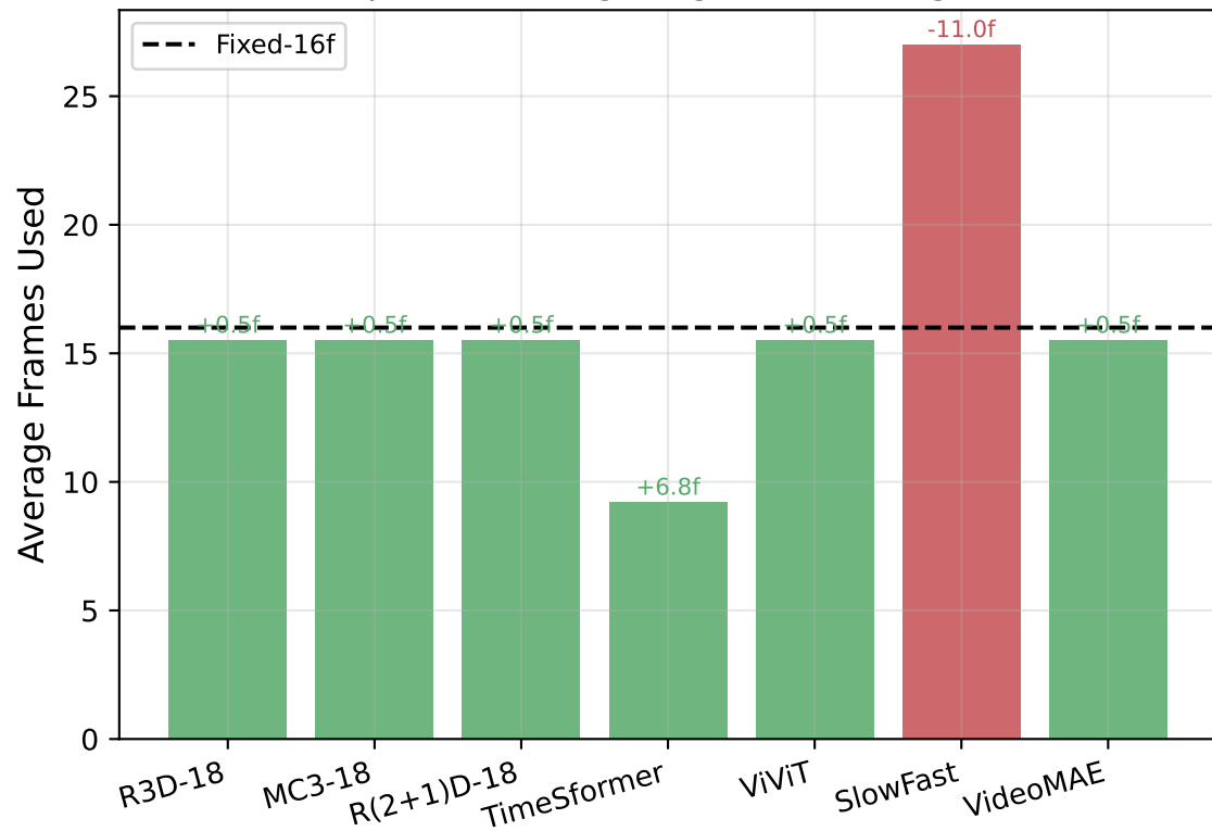
FDE Adaptive Routing: Avg Frame Budget (SSV2)
