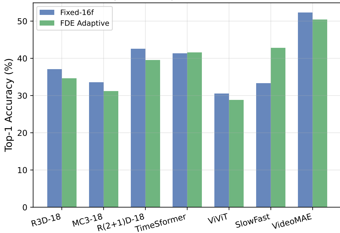
Accuracy: FDE Adaptive vs Fixed-16f (SSV2)
