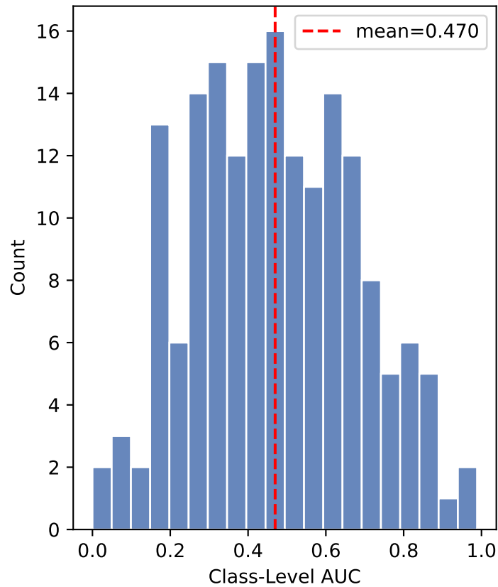
AUC Distribution VideoMAE on SSV2
