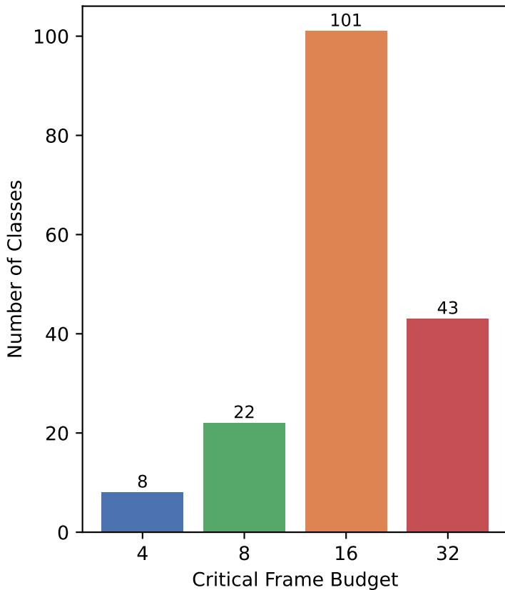
Critical Budget Distribution VideoMAE on SSV2
