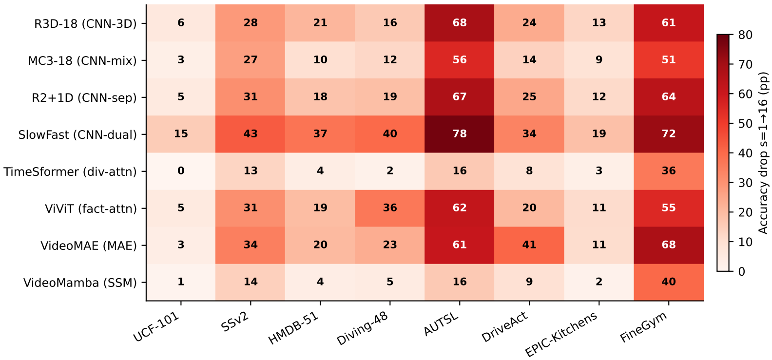
Fig 2: Temporal Aliasing Sensitivity — Accuracy Drop (stride 1→16, coverage=100%)
