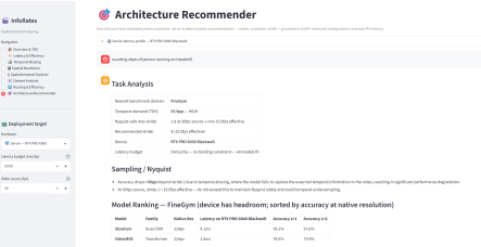
(c) Architecture Recommender: FineGym example. The system identifies FineGym as a high-TDS domain (55.9pp), requires stride \leq 2 , and ranks models by accuracy under the user's latency budget.
