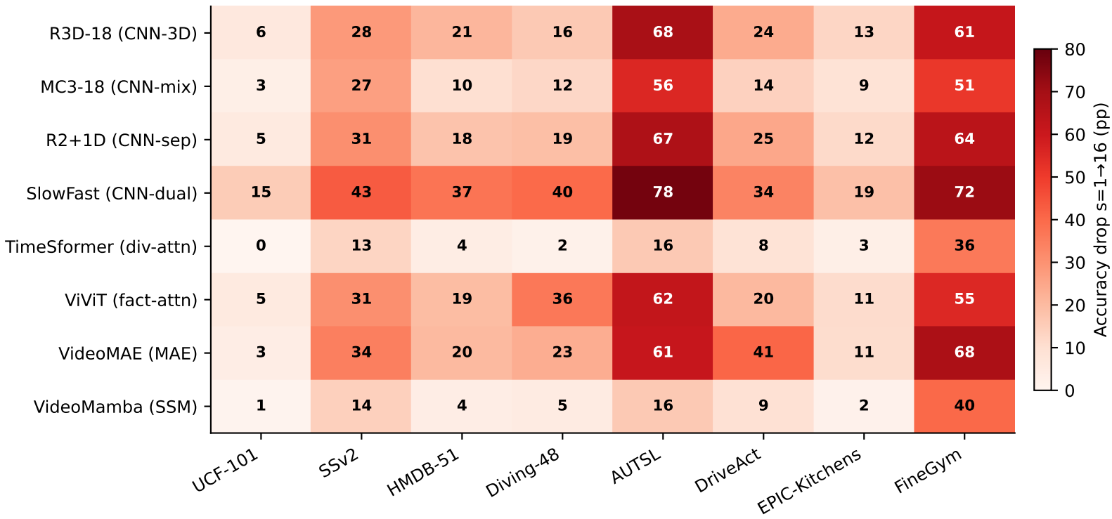
Fig 2: Temporal Aliasing Sensitivity — Accuracy Drop (stride 1→16, coverage=100%) † = feature collapse (s1<5%). VideoMamba/AUTSL uses native-res fine-tuned checkpoint.
