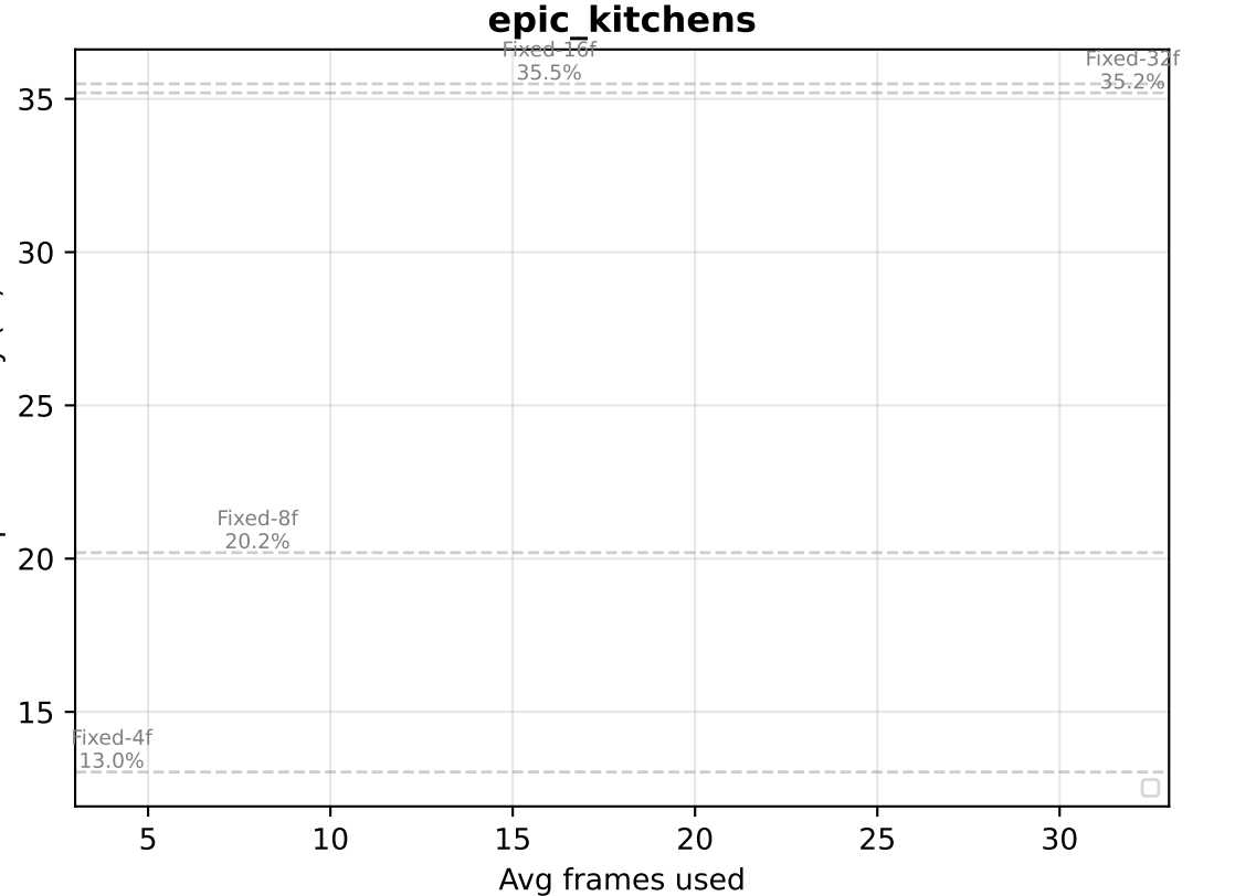
Confidence Cascade: Accuracy vs Avg Frames (vs fixed-budget baselines, dashed)
