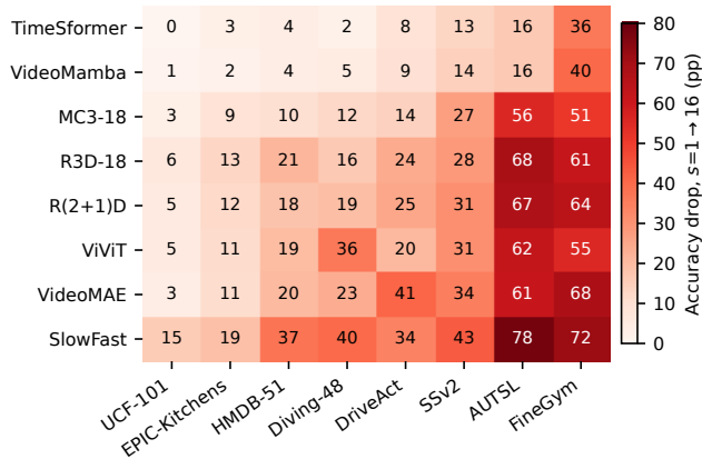
Fig. 5. Cross-architecture aliasing-loss heatmap: accuracy drop (pp) from stride=1 to stride=16 at cov=100%. Models are sorted top-to-bottom by increasing mean drop and datasets left-to-right by increasing TDS.
