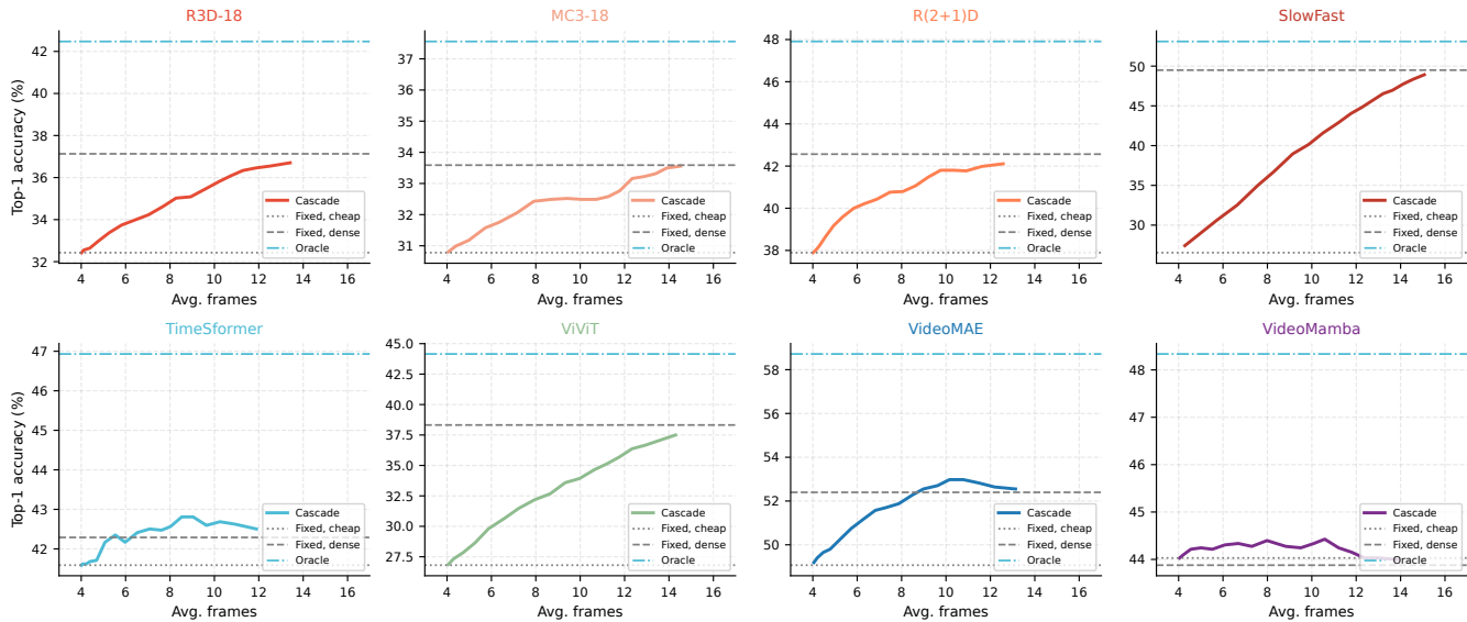
Fig. S12. Confidence cascade: accuracy vs. avg frames (SSv2, stride-4 cheap → stride-1 dense). For architectures with flat 4f≈16f accuracy (TimeSformer, VideoMamba), routing near-trivially selects 4f for most videos and matches dense accuracy. For architectures with large 4f–16f gaps (SlowFast, ViViT), the routing curve provides meaningful operating points between the fixed-budget extremes.
