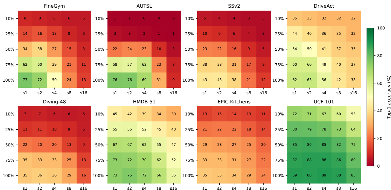
Fig. S3. R2+1D-18 (separable spatiotemporal convolution) heatmaps. Higher base accuracy than R3D-18 on several datasets (SSv2: 42.6% vs 37.1%), but similar aliasing sensitivity pattern—cliff at stride 4→8 on AUTSL and FineGym.
