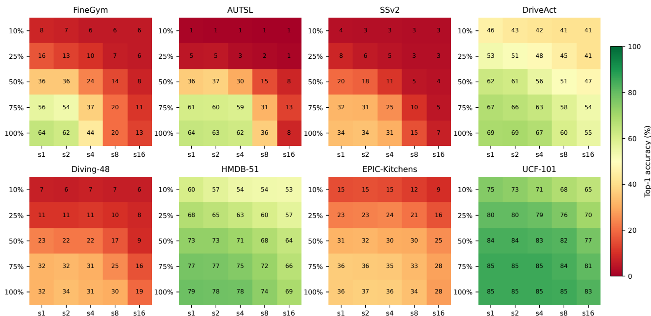
Fig. S2. MC3-18 (CNN-mix, channel-separated 3D) heatmaps. Similar pattern to R3D-18 but with slightly reduced aliasing on low-TDS datasets (UCF-101, DriveAct), consistent with the regularizing effect of 2D-channel separation. FineGym shows the same severe cliff pattern as AUTSL.
