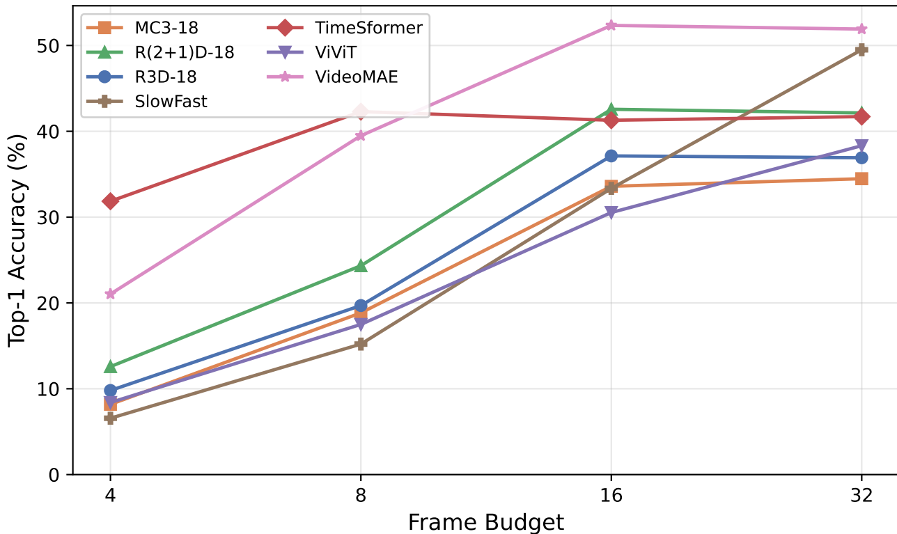
SSV2: Accuracy vs Frame Budget
