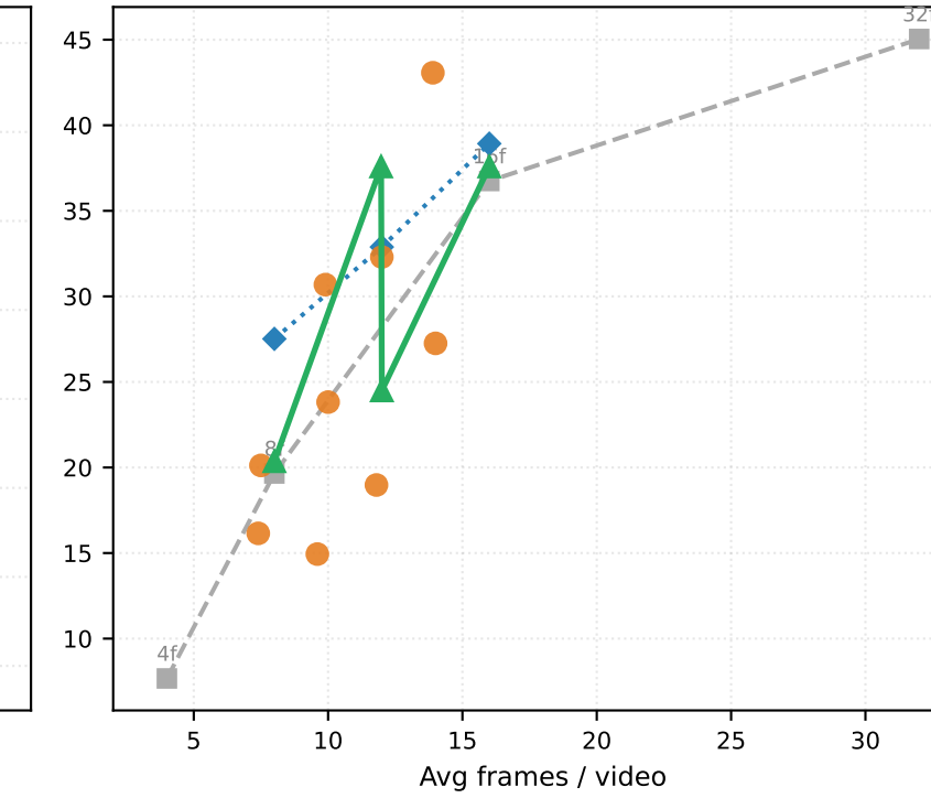
Diving48 (temporal-hard)
