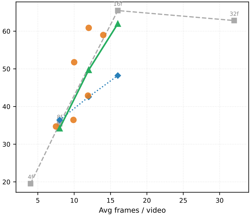
EPIC-Kitchens
