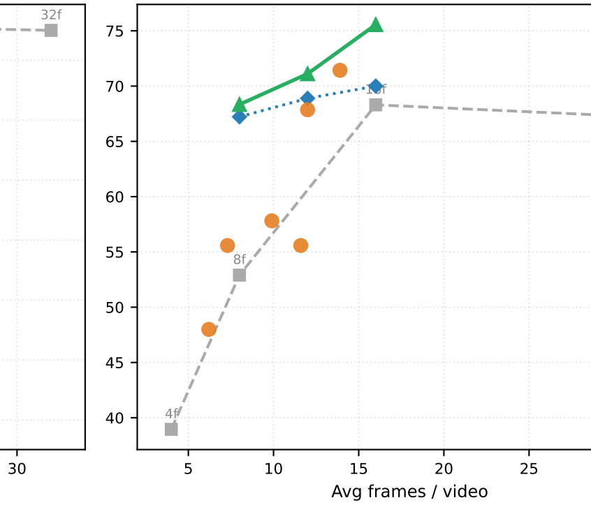
Drive&Act (driving)
