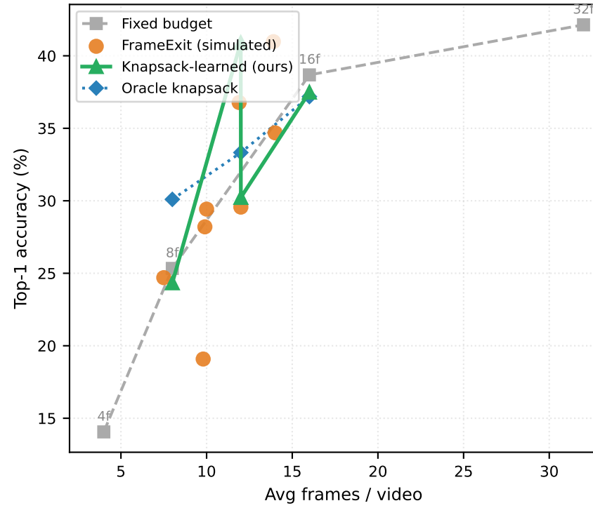
SSV2 (temporal-hard)
