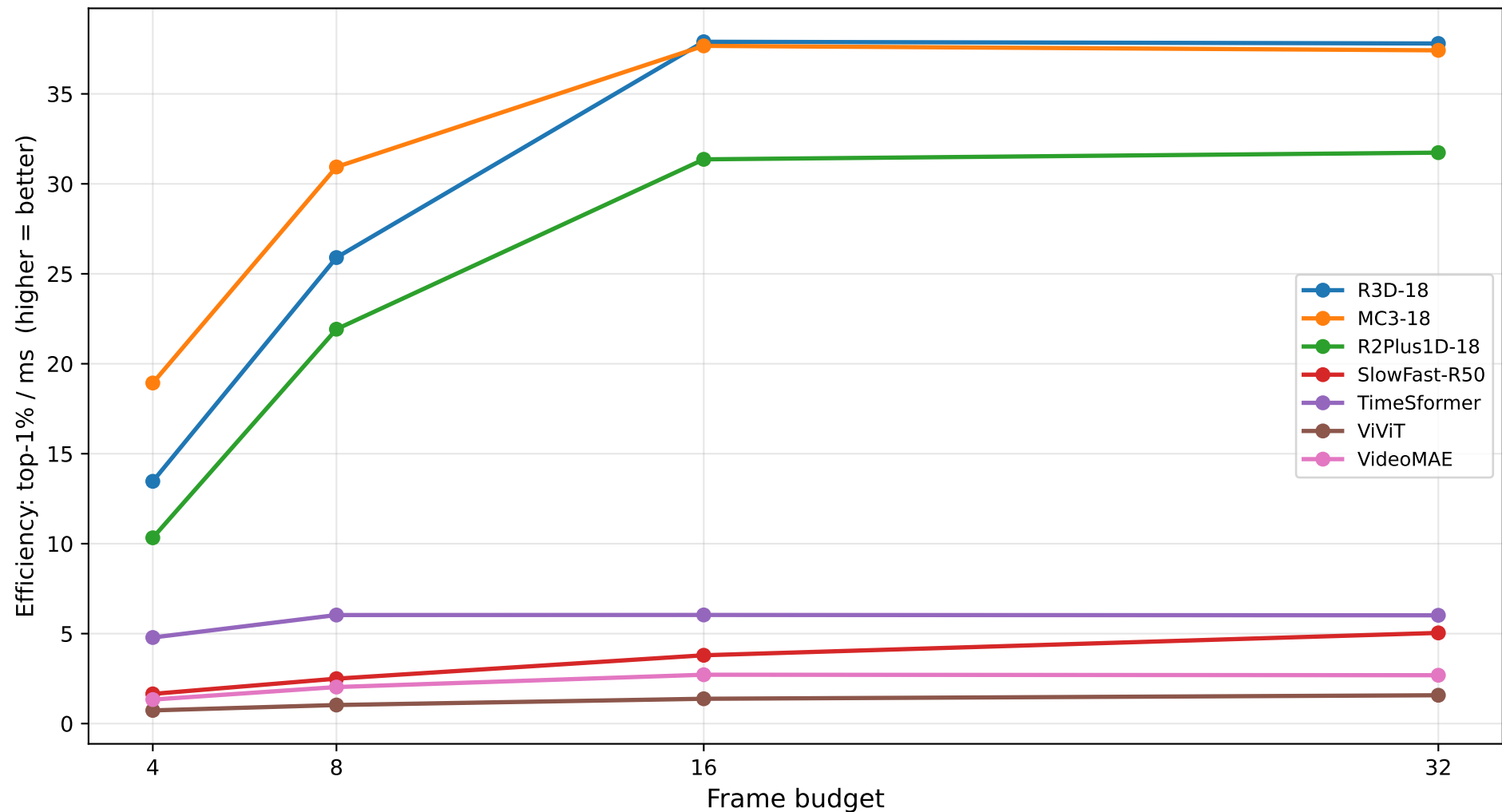
Accuracy-Efficiency Tradeoff by Model & Budget (mean across datasets)
