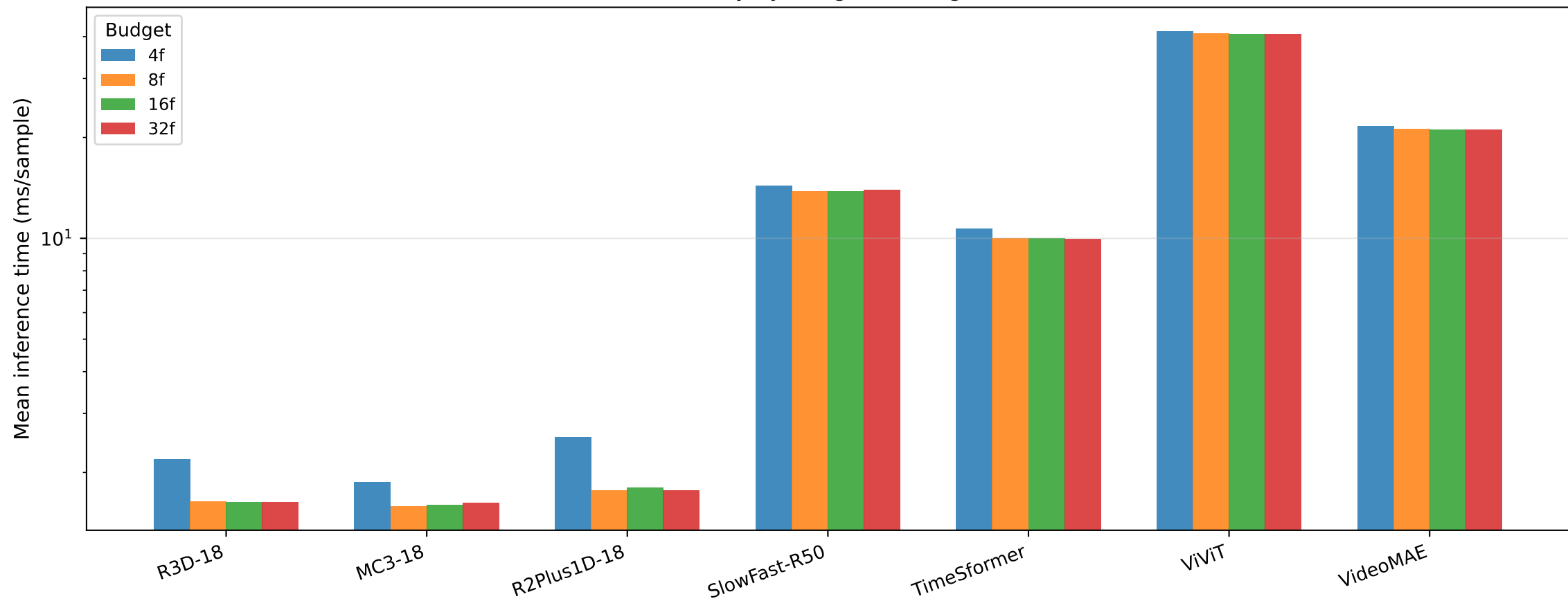
Model Inference Latency by Budget (averaged across datasets)
