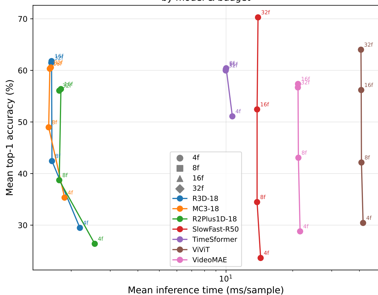
Accuracy vs Latency (averaged across datasets) by model & budget
