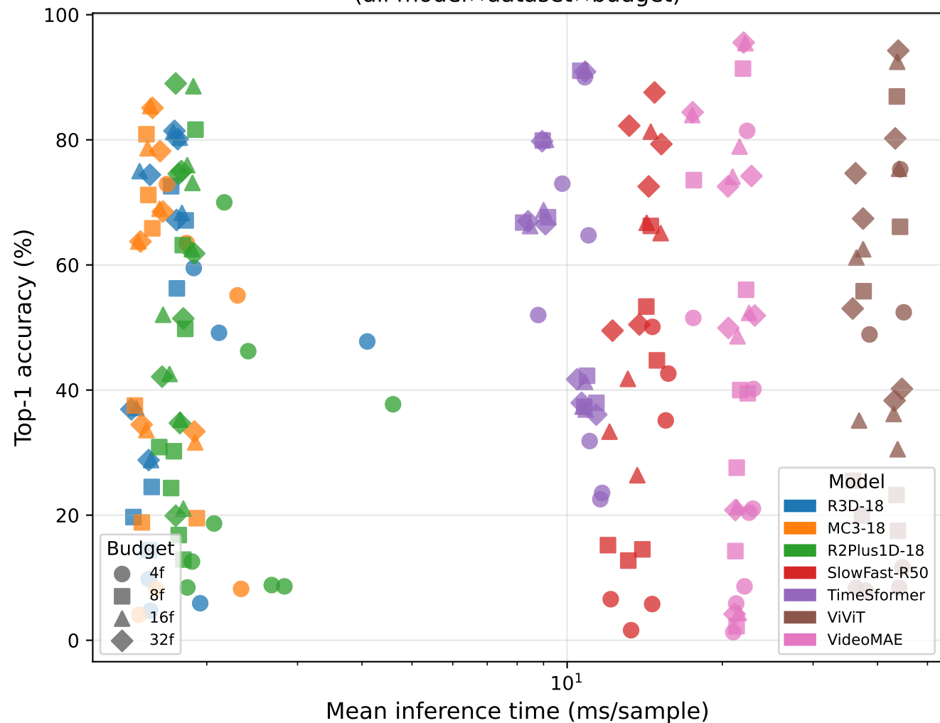
Accuracy vs Inference Latency (all model×dataset×budget)
