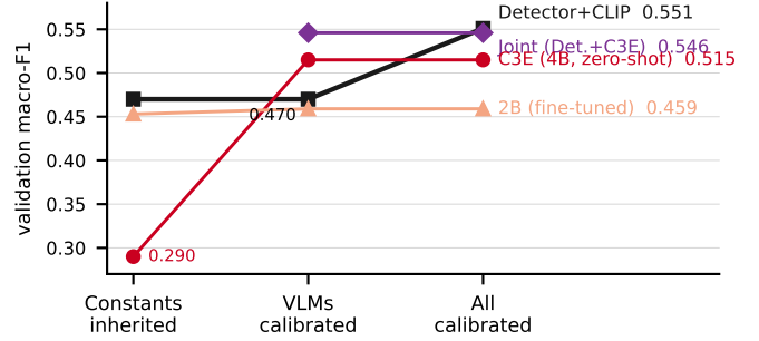
Fig. 1. The hidden variable. Validation macro-F1 (208 videos) under three comparison regimes. Left: every VLM runs the 2B’s temporal constants and the detector pipeline its published ones; the zero-shot 4B reasoner (C3E) looks useless. Middle: the VLM systems are calibrated and the baseline is not, as in a typical comparison; C3E and the joint estimator beat the detector pipeline. Right: the baseline is calibrated by the same procedure and becomes the best system.
