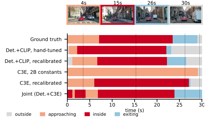
Fig. 3. Ground truth and five systems on one validation video, chosen to illustrate the effect; thumbnails mark the middle of each annotated state. With the 2B’s constants, C3E never leaves APPROACHING; recalibrated, it tracks the zone. The hand-tuned detector pipeline enters INSIDE 5 s early and cuts EXITING short; recalibrated, it follows all four states.
