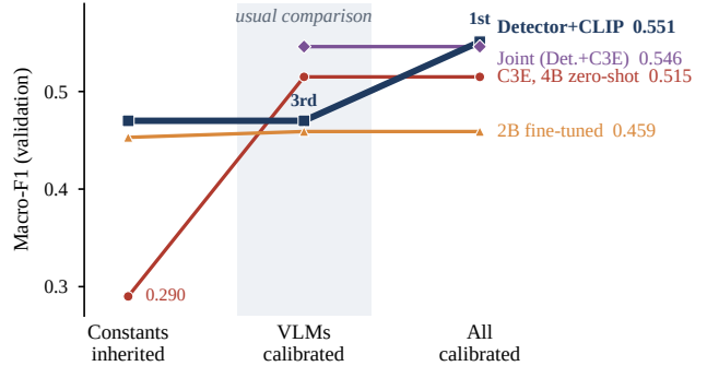
Fig. 1. The hidden variable. Validation macro-F1 (208 videos) under three comparison regimes. Left: every VLM runs the 2B’s temporal constants and the detector pipeline its published ones; the zero-shot 4B reasoner (C3E) looks useless. Middle: the VLM systems are calibrated and the baseline is not, as in a typical comparison; C3E and the joint estimator beat the detector pipeline. Right: the baseline is calibrated by the same procedure and becomes the best system.
