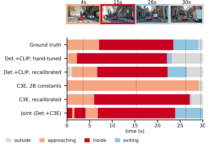
Fig. 2. Ground truth and five systems on one validation video, chosen to illustrate the effect; thumbnails mark the middle of each annotated state. With the 2B’s constants, C3E never leaves APPROACHING; recalibrated, it tracks the zone. The hand-tuned detector pipeline enters INSIDE 5 s early and cuts EXITING short; recalibrated, it follows all four states.
