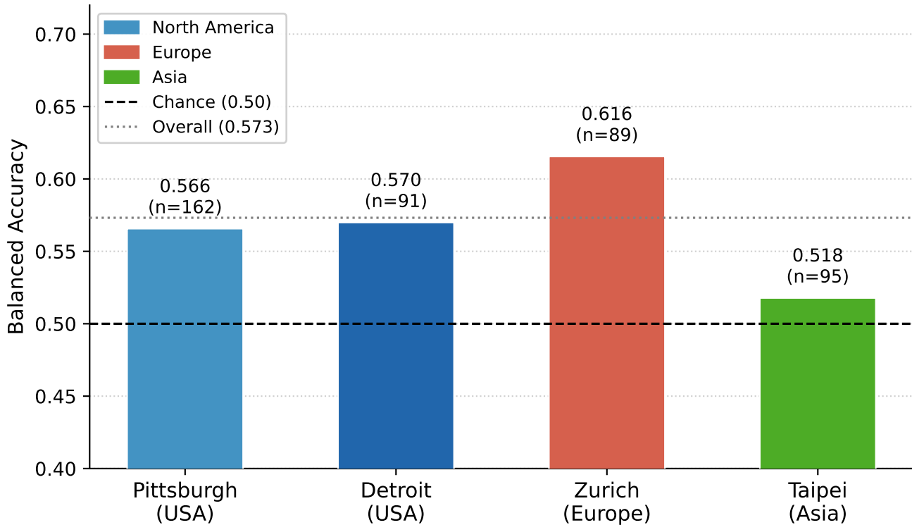
Generalization: DINOv2-large across unseen cities (trained on Pittsburgh passability votes, tested on CurbRamp/NoCurbRamp labels)
