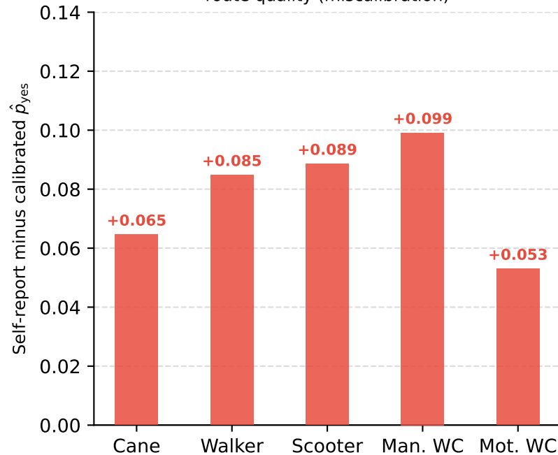
(b) Hard-CE overestimates own route quality (miscalibration)
