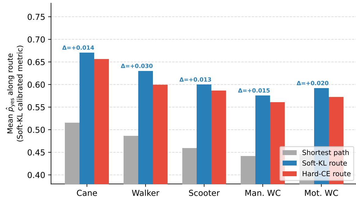
(a) Routing quality — Soft-KL beats Hard-CE on every aid (calibrated evaluation)
