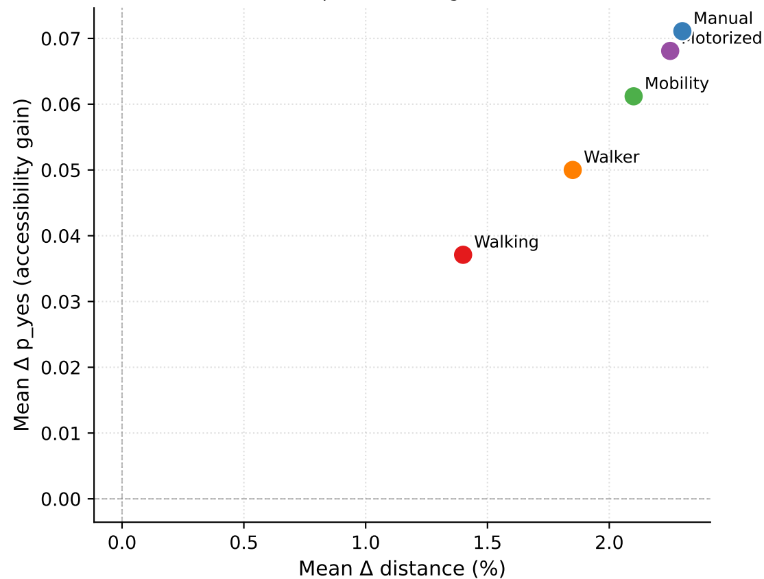
Accessibility gain vs. distance overhead 10,000 OD pairs, Pittsburgh PA (bc=1.0)
