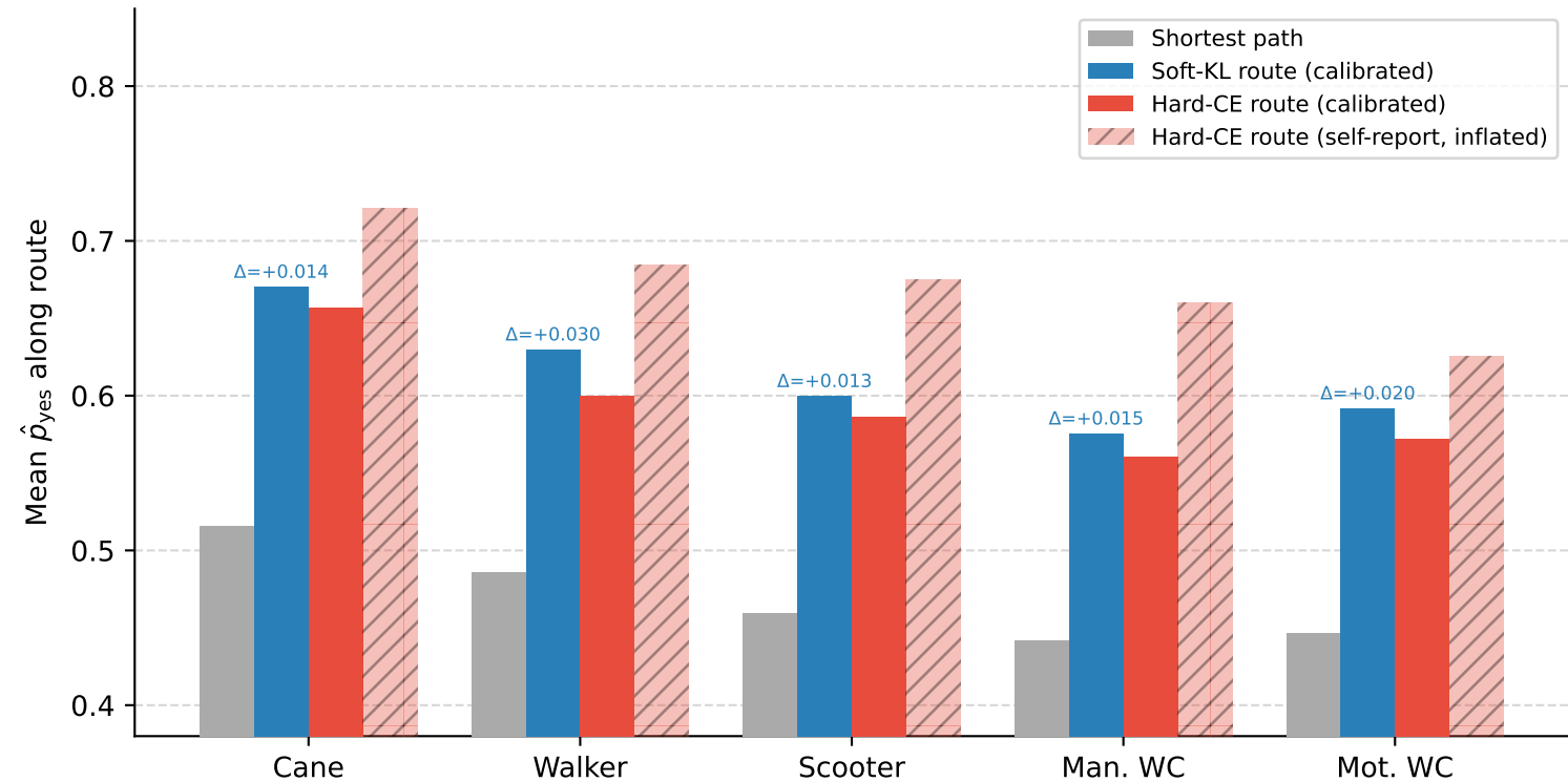
Routing quality: Soft-KL vs Hard-CE edge scores (evaluated by calibrated Soft-KL metric — ground truth)
