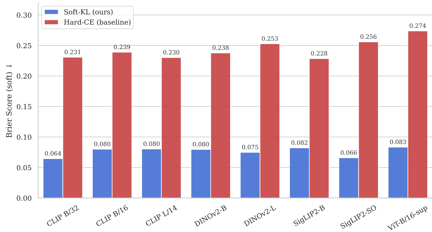
Calibration Quality: Soft-KL vs Hard-CE Brier score against human vote distributions — lower is better
