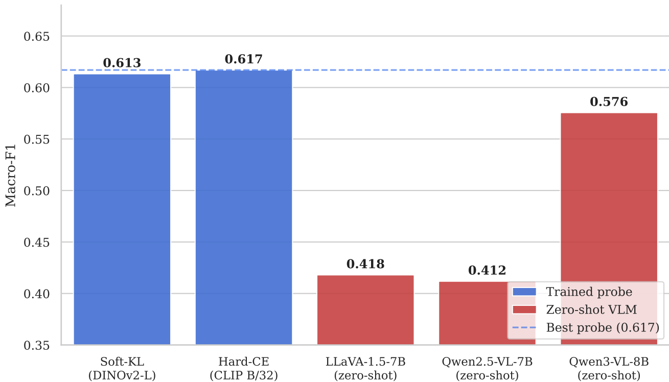
Trained Probe vs Zero-Shot VLMs Overall Macro-F1 (5 mobility aids)
