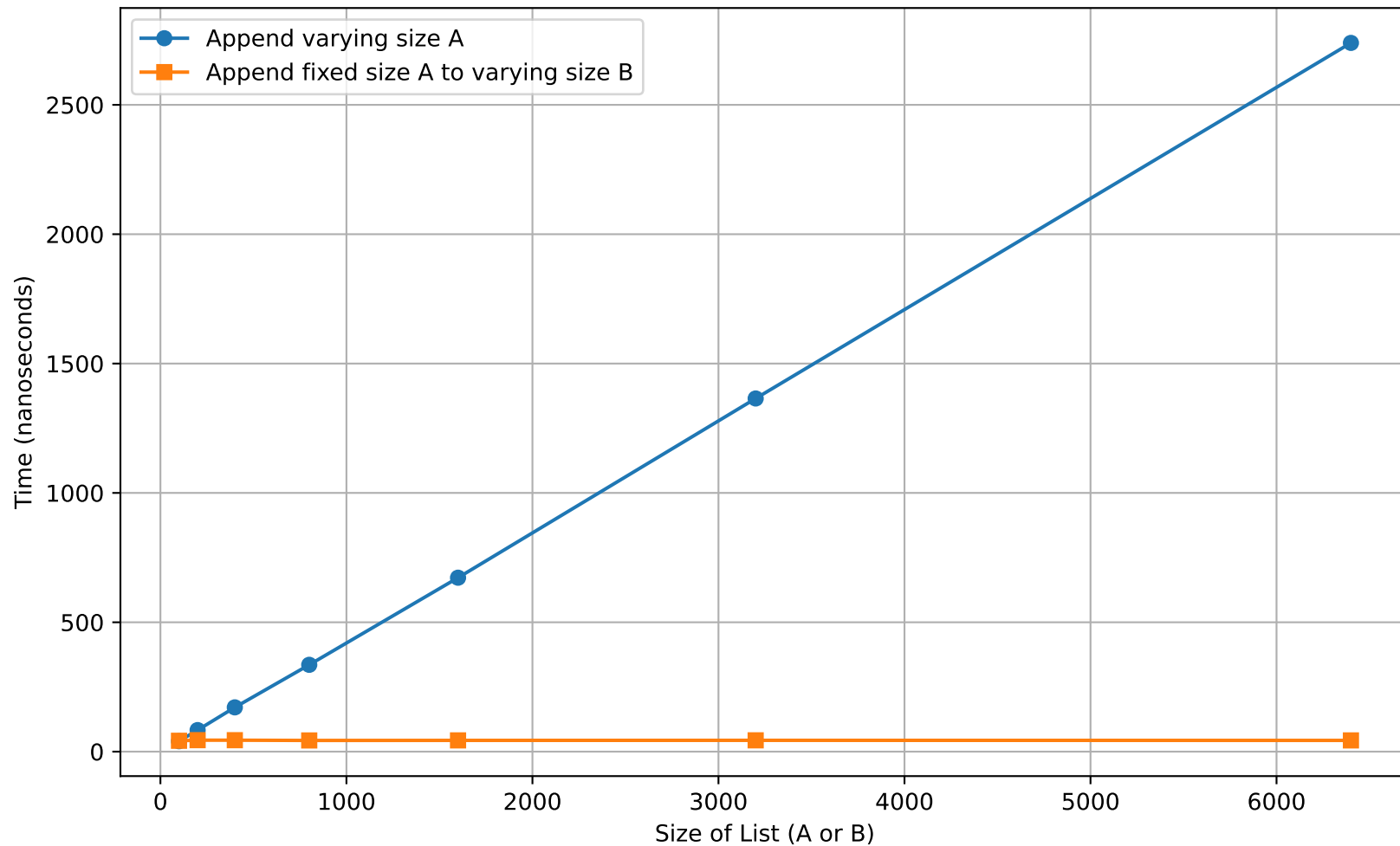
Benchmarking Linked List Append Operation
