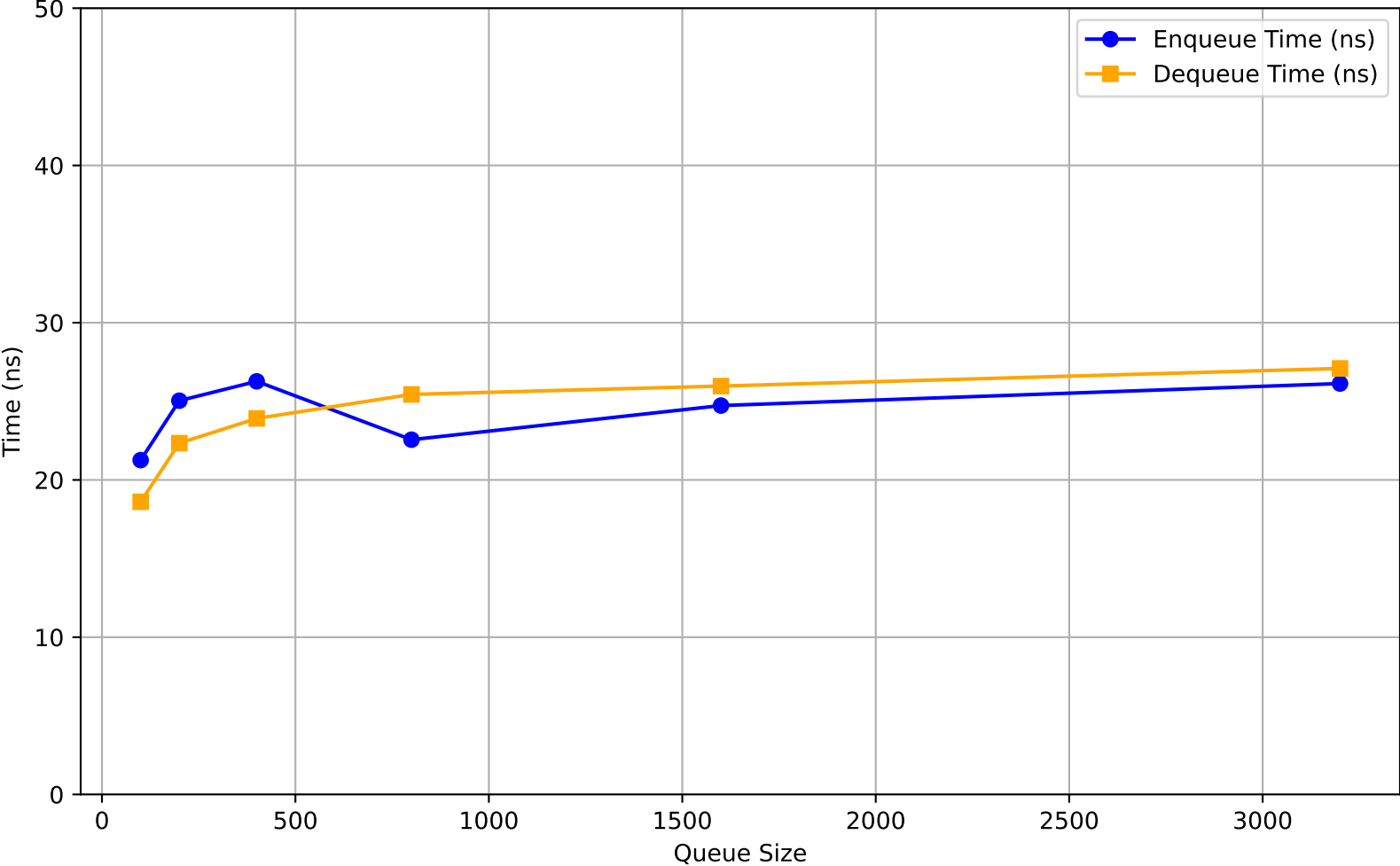
Improved Queue Benchmark Result
