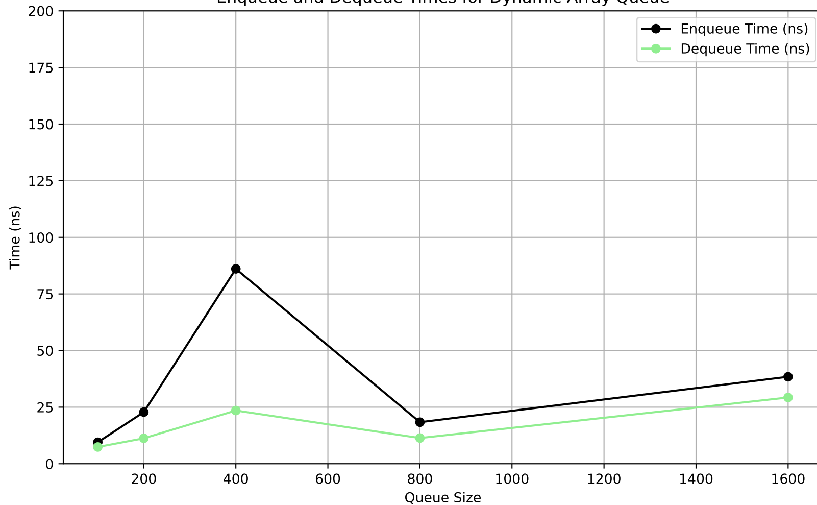
Enqueue and Dequeue Times for Dynamic Array Queue
