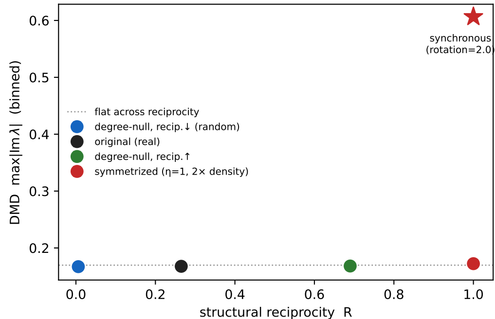
(a) symmetry readout is blind to reciprocity
