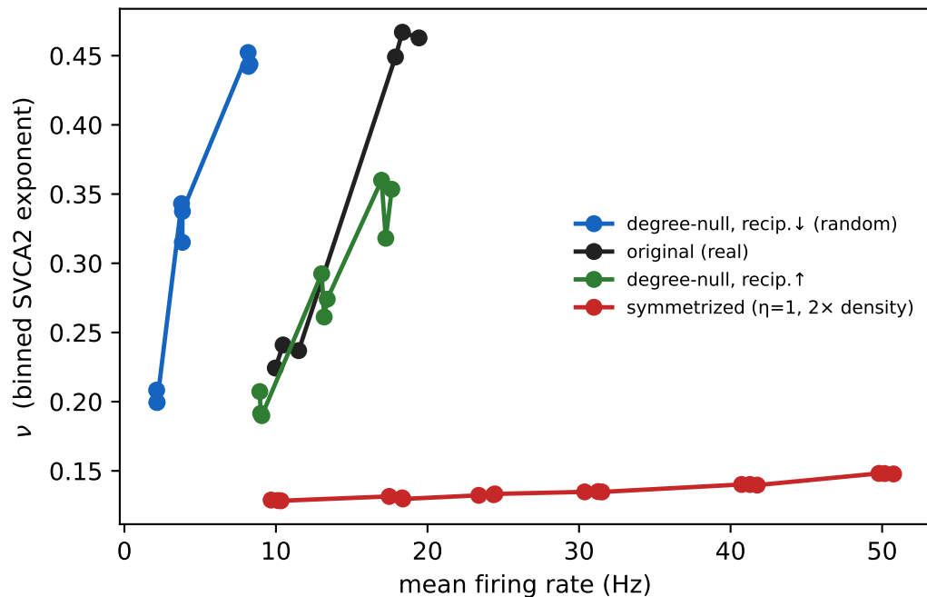
(b) \nu : symmetrized flat = density, not reciprocity
