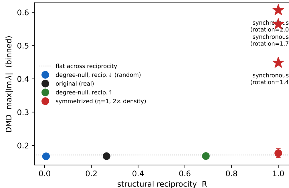
(a) symmetry readout is blind to reciprocity
