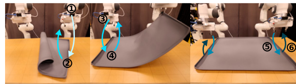
Figure 10. Bimanual mat unrolling. The robot needs to ① pick up one side of the mat (if needed), using the left or right arm, ② lift and unroll the mat (if needed), ③ ensure that both sides of the mat are grasped, ④ lift the mat, ⑤ place the mat oriented with the table, mostly centered, and ⑥ release the mat.
