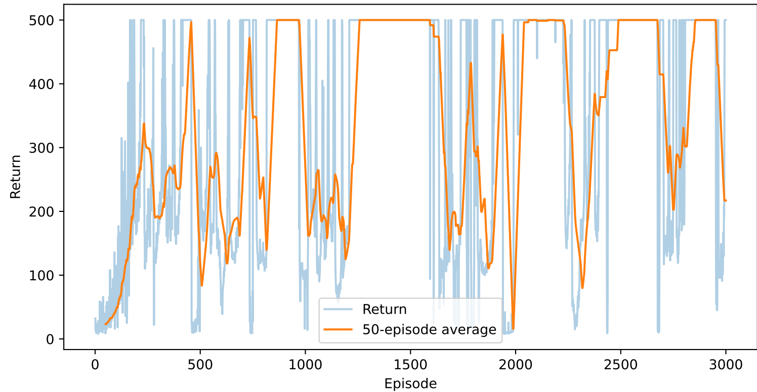
Online one-step Actor-Critic on CartPole-v1
