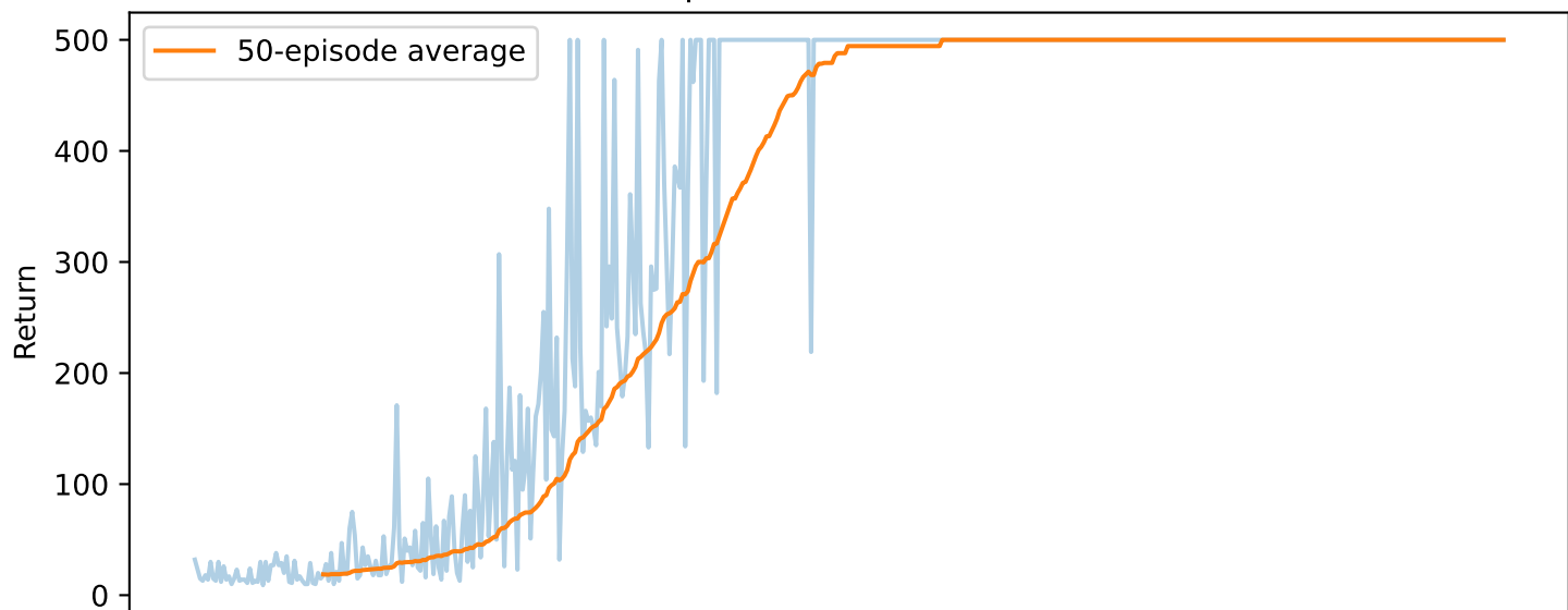
PPO-Clip with GAE on CartPole-v1
