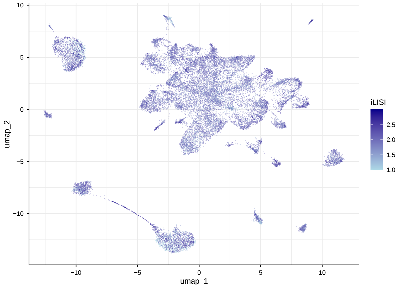
iLISI score (integration of three samples)
