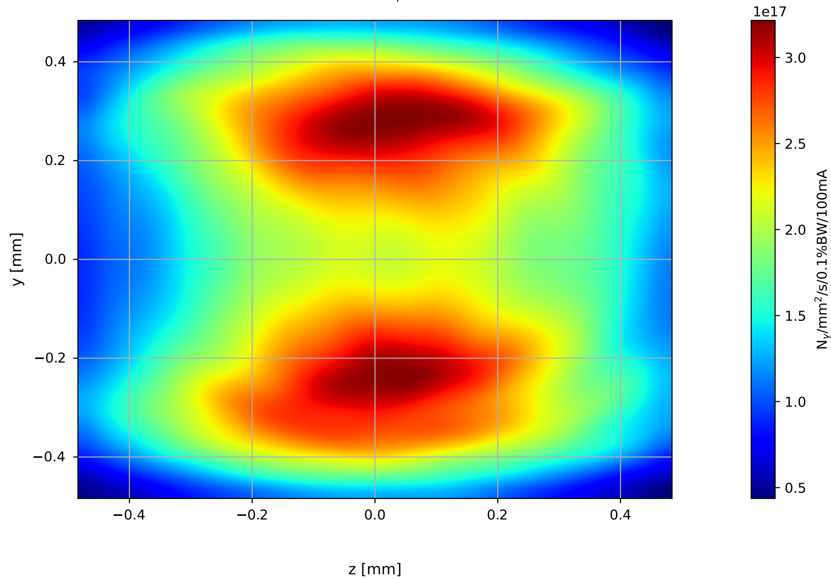
Dens. of S_0 for E_\gamma = 698 eV
