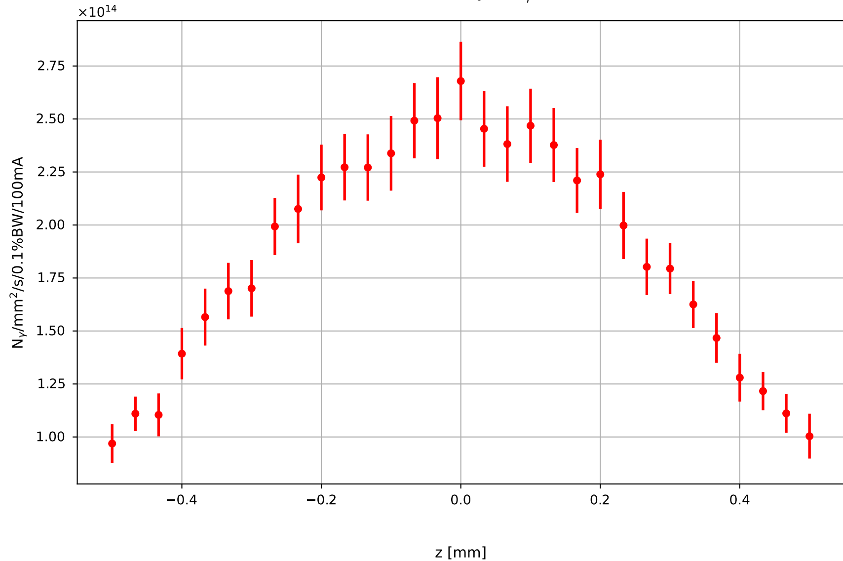
Horizontal Profile of S_0 for E_\gamma = 699 eV
