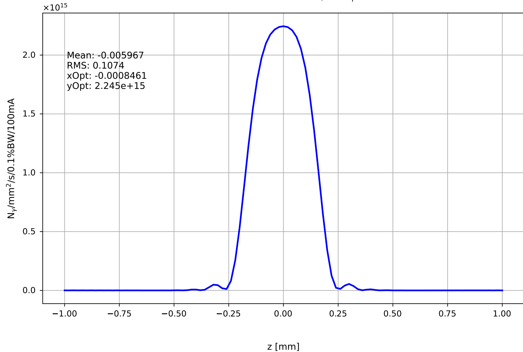
Horizontal Cut at x = 10.0\text{m} of S_0 for E_\gamma = 700\text{ eV}
