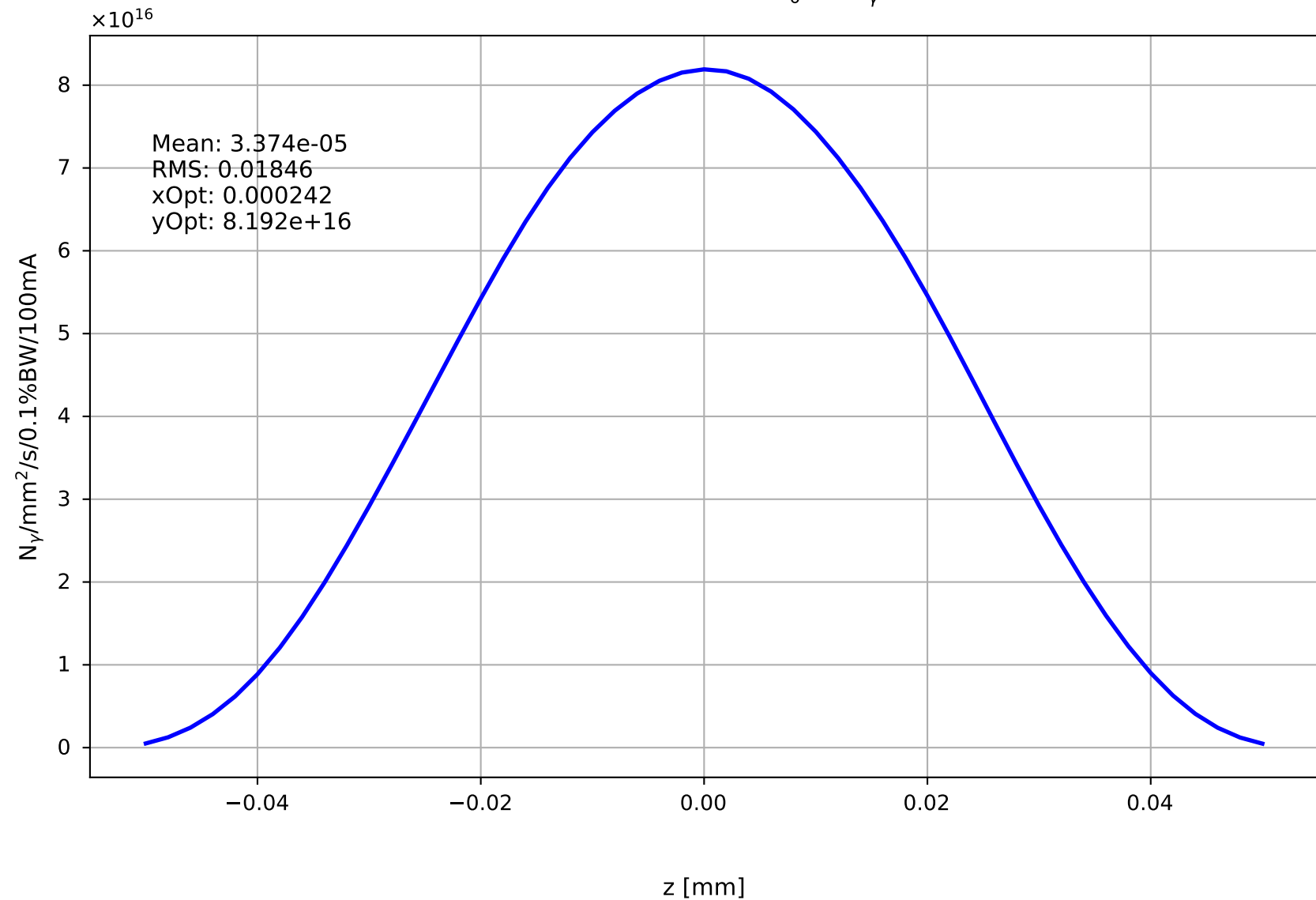
Horizontal Cut at x = 0.0\text{m} of S_0 for E_\gamma = 700\text{ eV}
