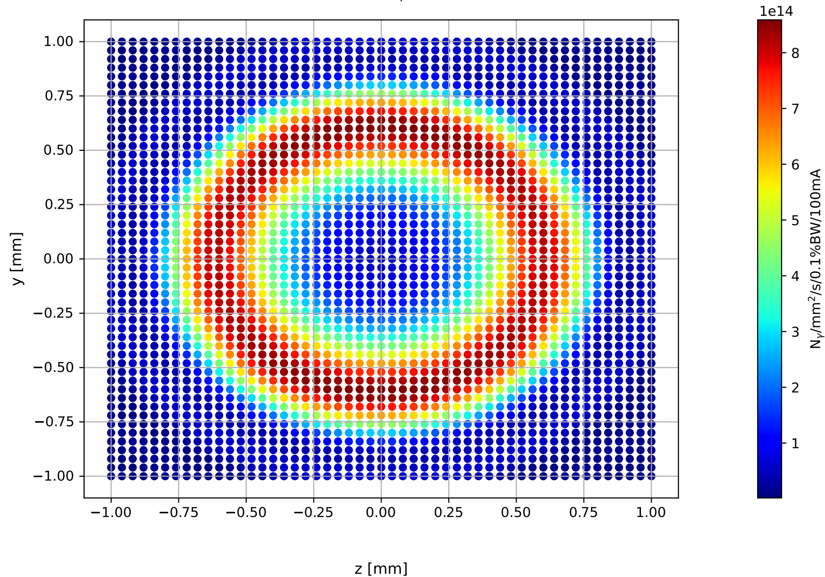
Dens. of S_0 for E_\gamma = 99.2 eV
