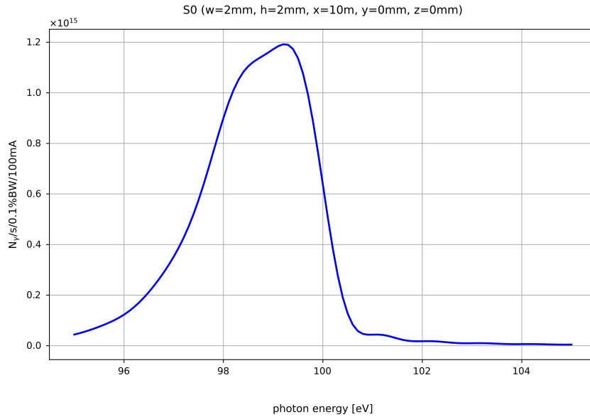
Fig. 3: Flux of Undulator
