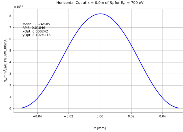
Fig. 14: Horizontal cut of S_0 in source plane
