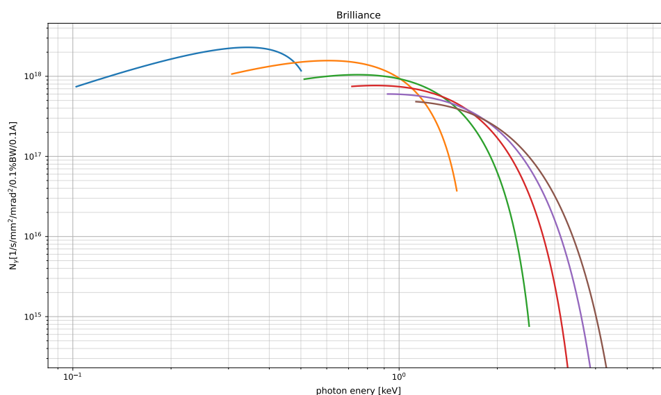
Fig. 2: Brilliance Plot
