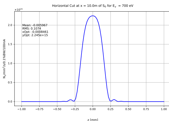
Fig. 13: Horizontal cut of S_0 in observation plane
