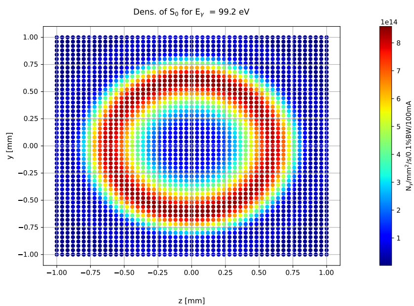
Fig. 4: Flux-density Distribution
