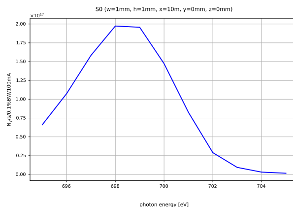
Fig. 6: Flux spectrum
