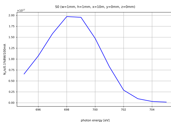
Fig. 6: Flux spectrum
