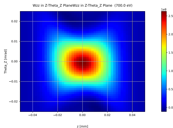
Fig. 15: Wigner distribution in source plane
